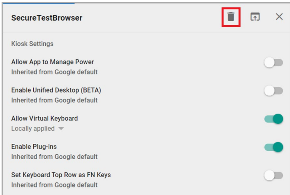
Figure 6. App Settings
